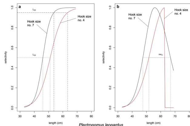
Fig. 6. Selectivity curve of Plectropomus leopardus using (A) asymptotic selectivity and (B) bell-shaped selectivity model by Hoshino et al. (2020). Adapted from Hoshino et al. (2020) with permission of Elsevier. For both selectivity curves, black solid line represents curve for hook number 7 and red solid line represents curve for hook number 4.
