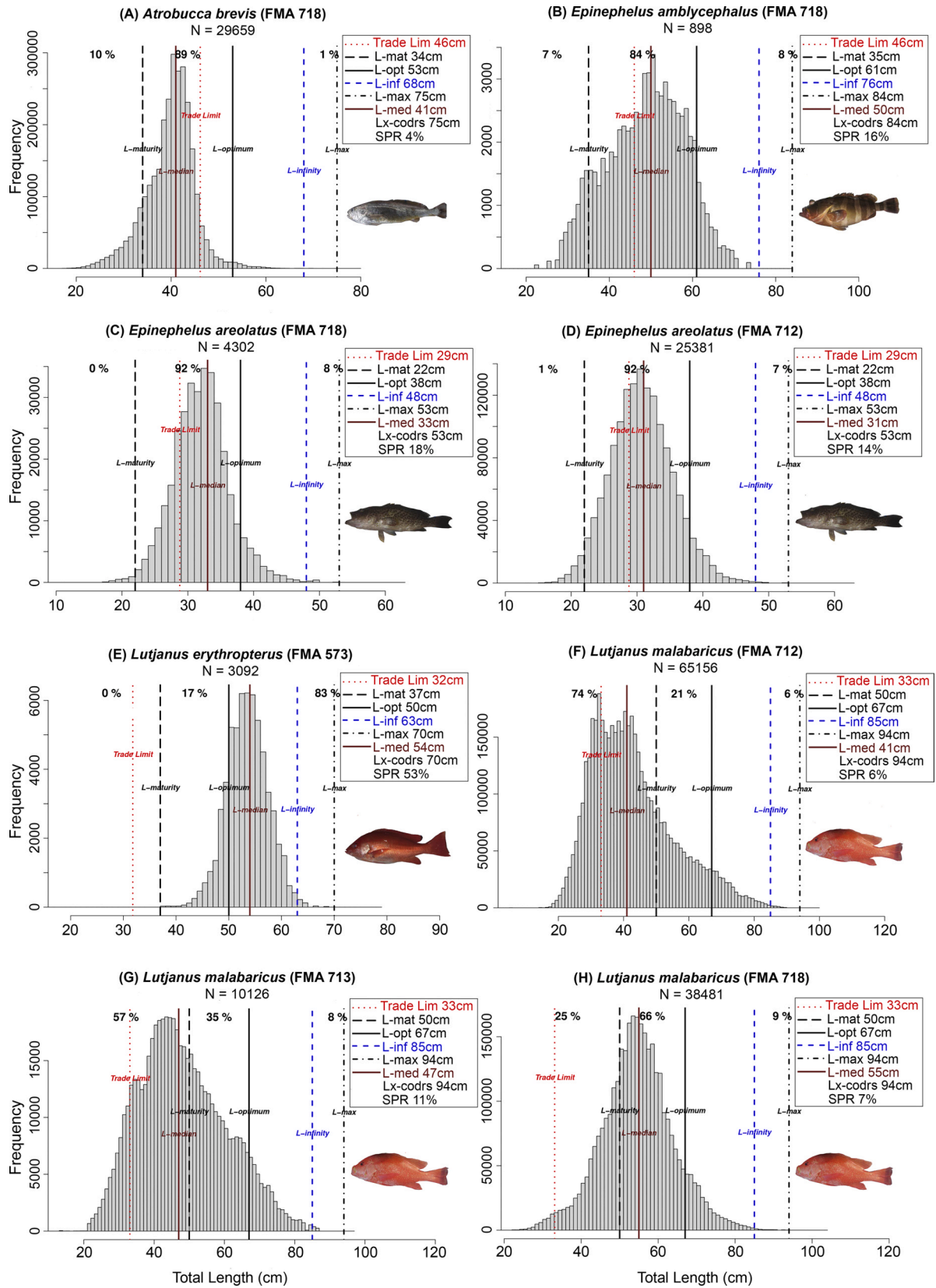
Fig. 2. Catch length frequency distributions, life-history parameters and reference points as estimated with the highly customized length-based approach presented here for orange croaker Atroubucca brevis (FMA 718), banded grouper Epinephelus amblycephalus (FMA 718), areolate grouper E. areolatus (FMAs 712 and 718), crimson snapper Lutjanus erythropterus (FMA 573), and Malabar red snapper L. malabaricus (FMAs 712, 713, 718). Fish photos are from the crew-operated data recording system (CODRS; Wibisono et al., 2019). SPR: spawning potential ratio. Lx-codrs = L_{max} , i.e. the largest specimen in the CODRS database.
